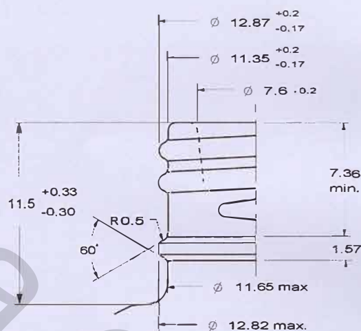
PRINTING SLOT DETAIL A
