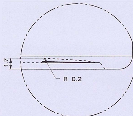
PRINTING SLOT DETAIL A
